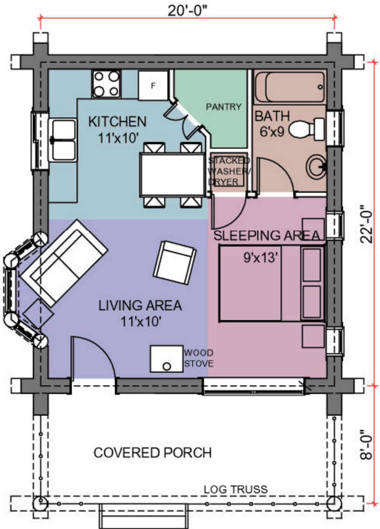
MAIN FLOOR PLAN AREA: 484 SQ. FT.
