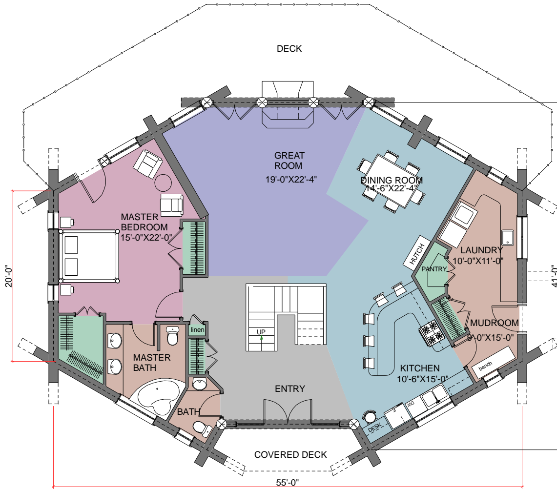
FIRST FLOOR PLAN AREA: 1858 SQ. FT.
